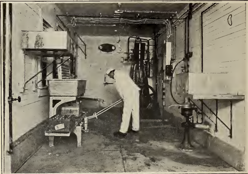
This cut shows Cream Separator, Ice Machine, Brine Cooler and exterior of Cold Storage Room.
